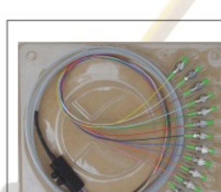
带状尾纤 Ribbon pigtails
